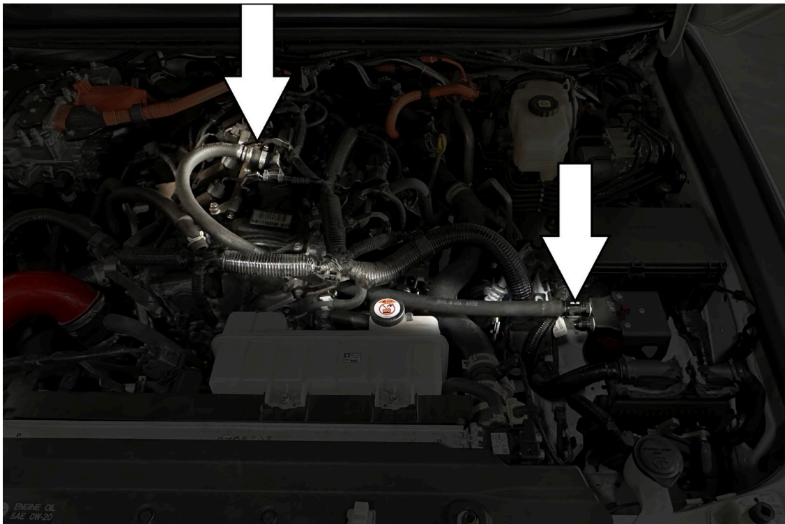
8. Install the pre-assembled 33-inch long hose from the valve cover to the oil catch can. Use the provided embossed hose clamp to secure the hose at the valve cover.
