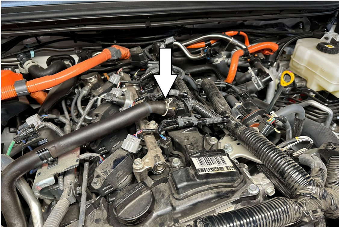
7. Disconnect the ventilation hose located at top of the engine.
