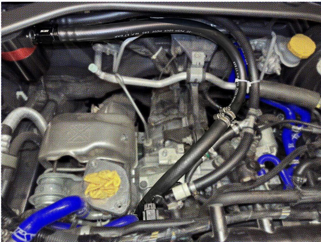
18. Push the AN-10 hose end fitting onto the AN-10 hose. Thread the hose end fitting onto the adapter on the oil catch can and fasten it securely.
