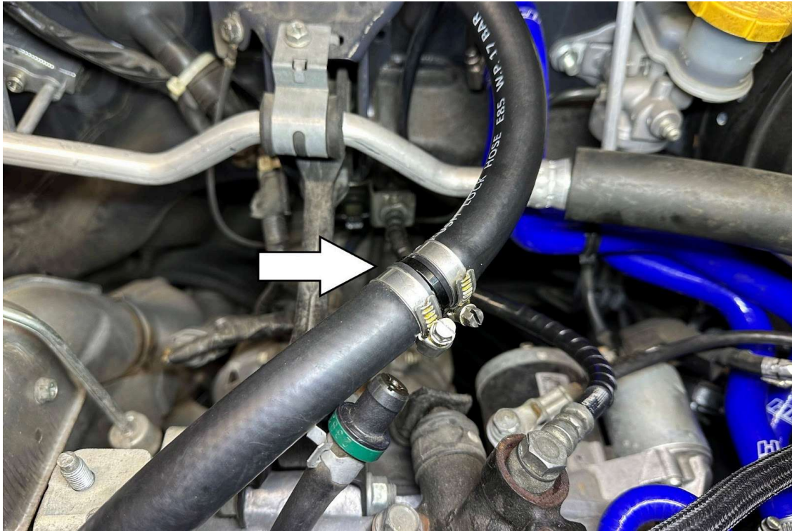
17. Install the 5/8" to 3/4" union to the AN-12 hose and install the AN-10 hose to the other side. Then secure them using two provided 16-27mm hose clamps.
