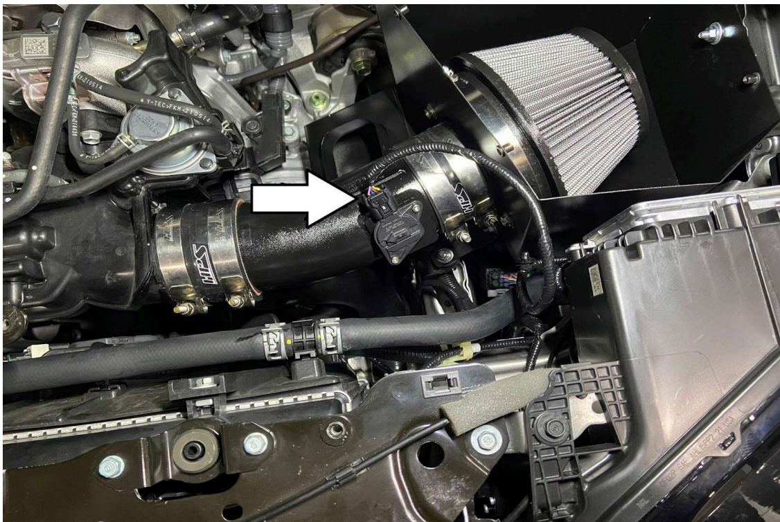
18. Reconnect the mass air flow sensor harness connector.
