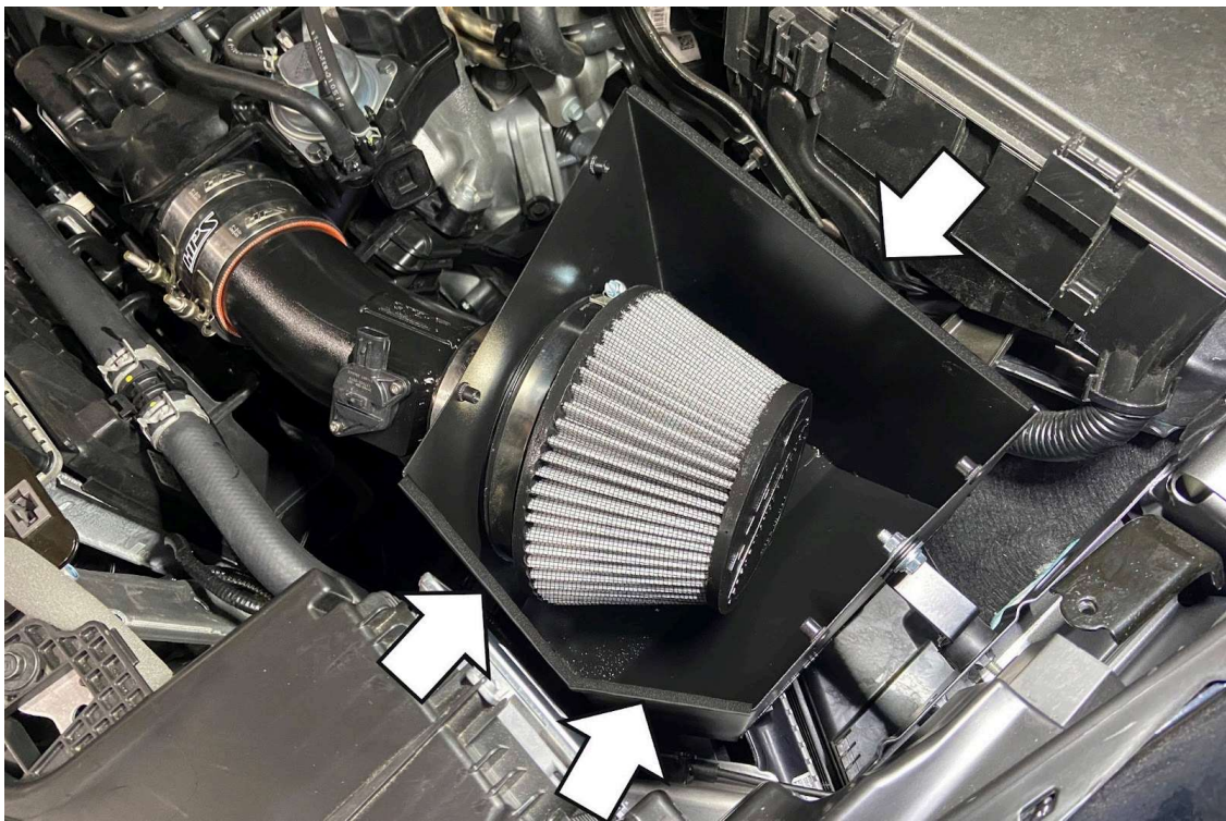
20. Install the edge trim onto the heat shield in the sections indicated in the image above.
