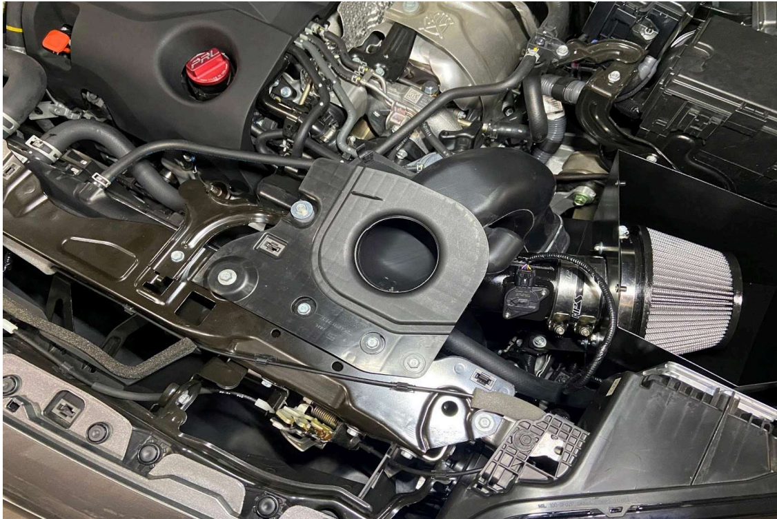
19. Reinstall the factory air duct back into the vehicle.
