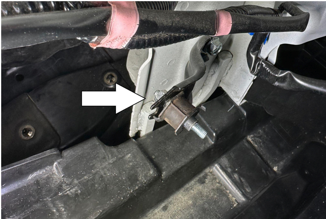
10. Loosen the nut to remove the rubber isolator from the vehicle.
