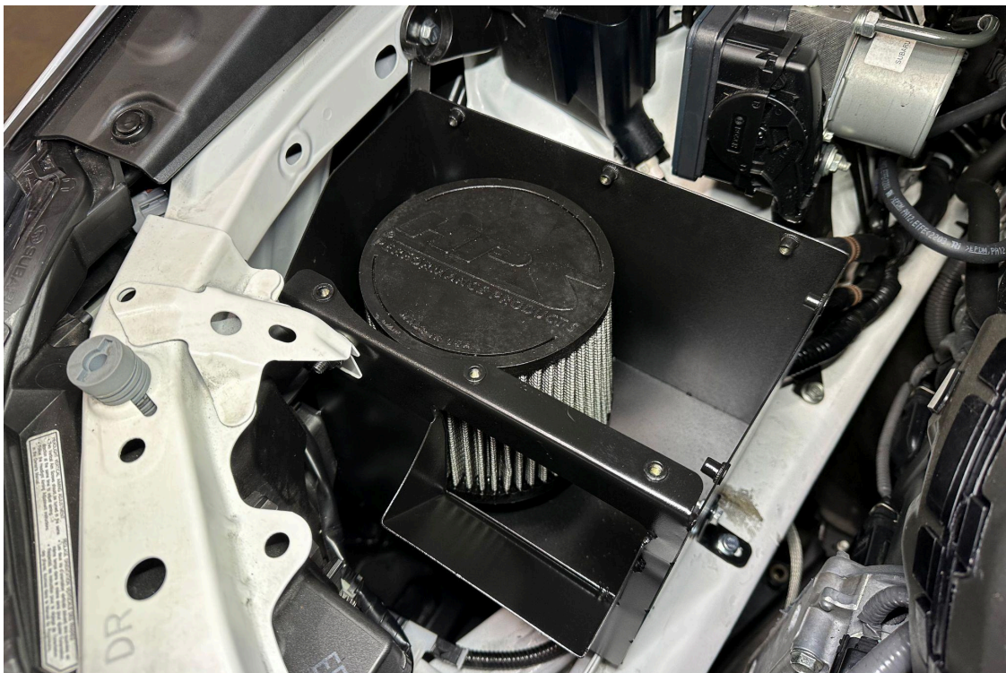
24. Install the provided HPS performance air filter using a ratchet and 8mm socket.
