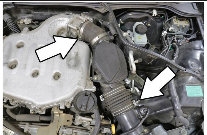
5. Loosen the hose clamps securing the intake tube from the throttle body and the factory MAF housing.
