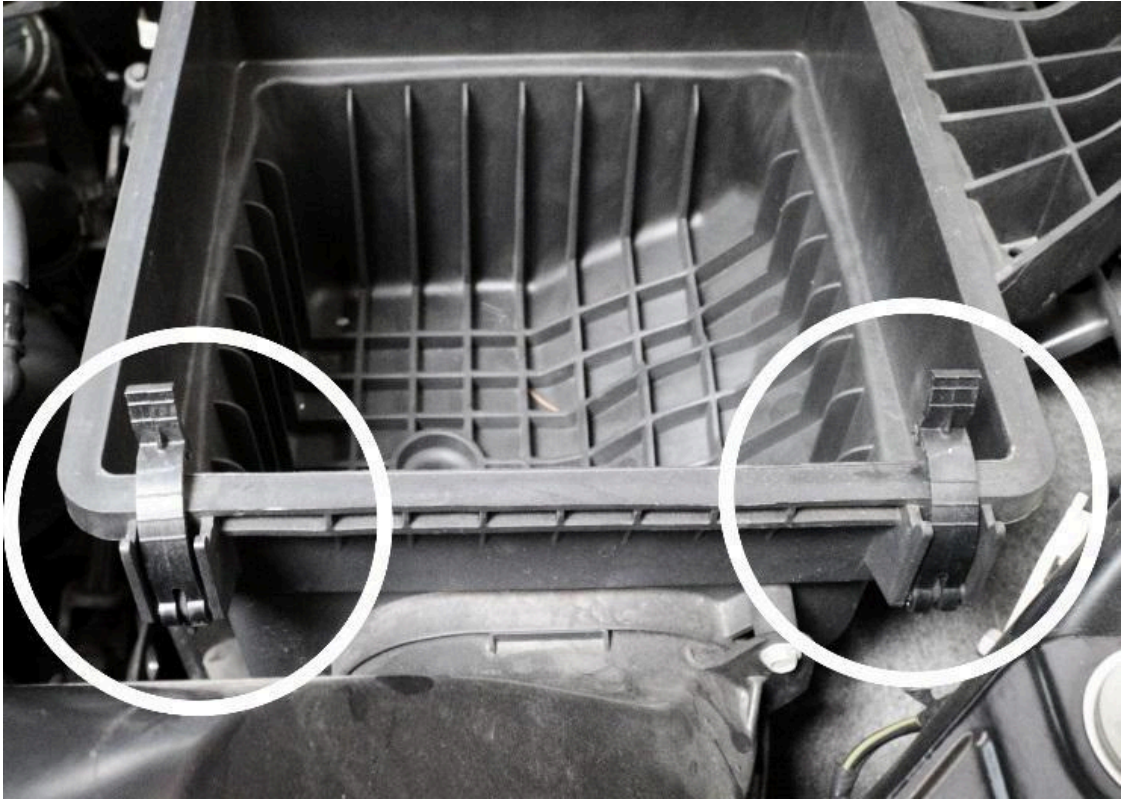
10. Push up the air box buckles.
