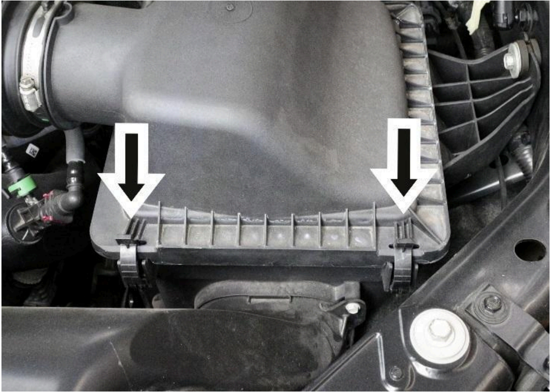
4. Unclip the air box buckles.
