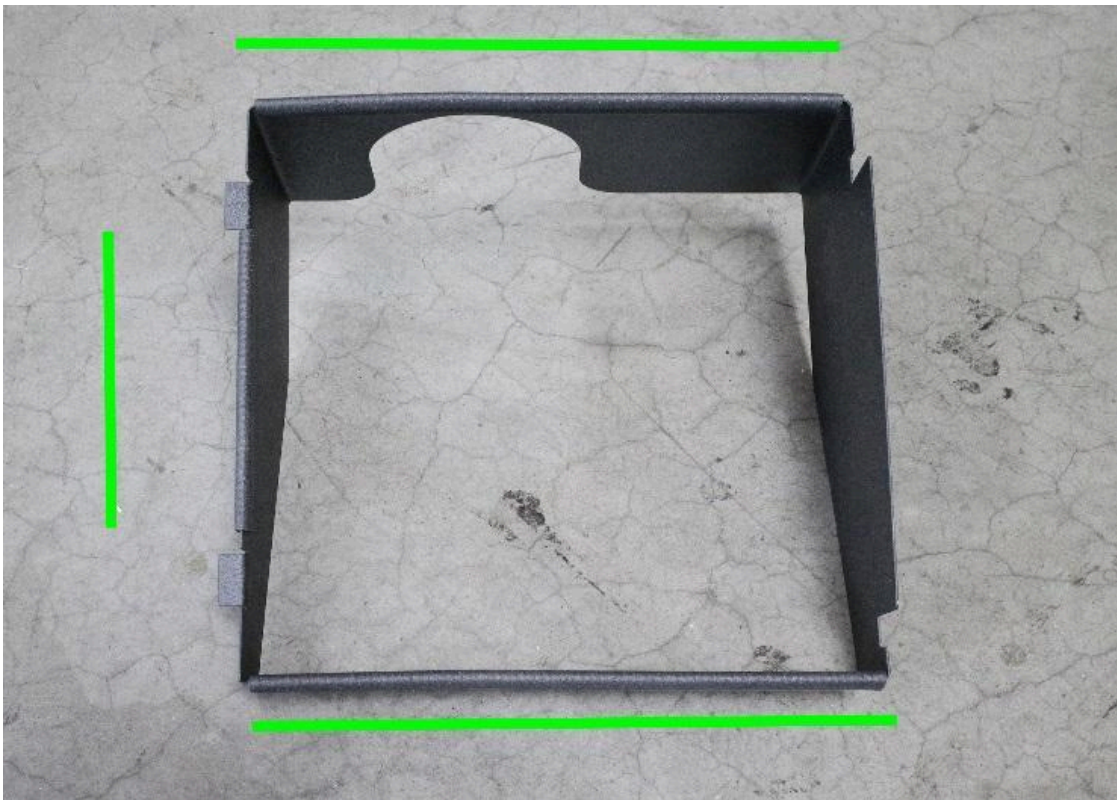
7. Install the thin edge trim onto the bottom side of the heat shield. Measure and cut to fit each section indicated above.
