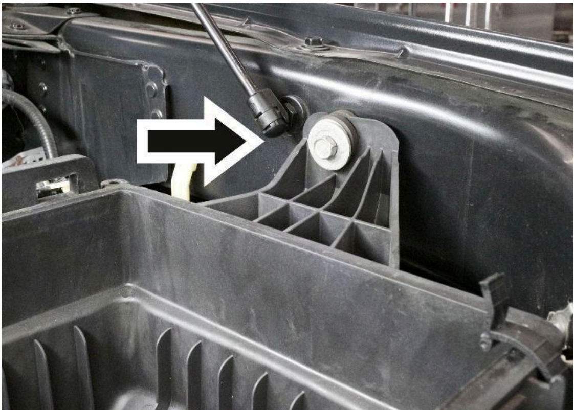
9. Loosen and remove the bolt securing the lower air box.
