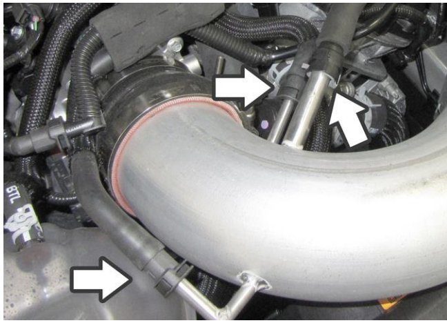
21. Re-connect the air hoses until they click into place.
