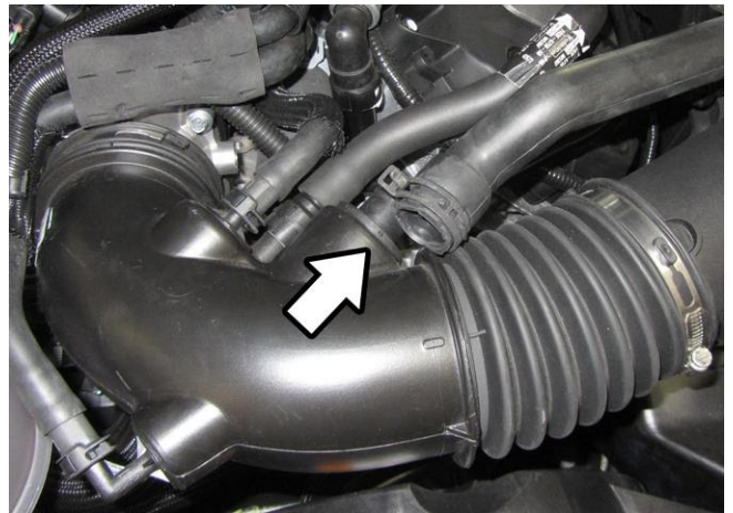
3. Pinch and release the spring clamp to disconnect the sound tube from the intake tube.
