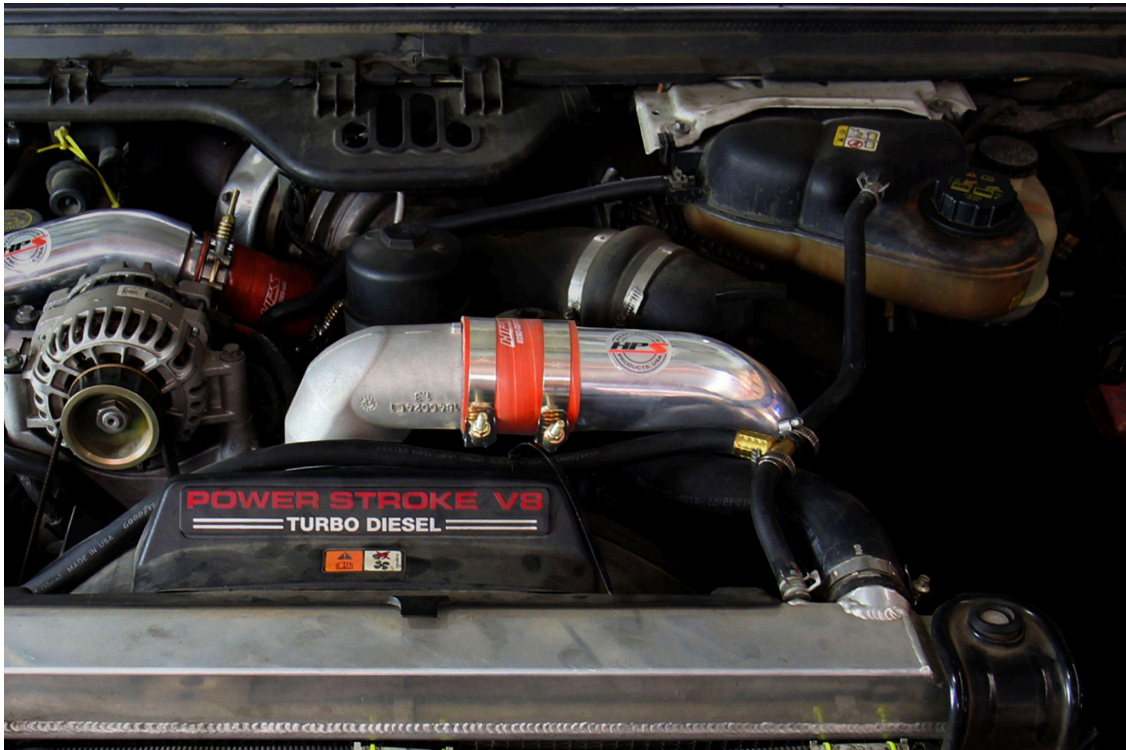
9. Tighten all of the clamps to 35 in-lb. to secure the pipe and hoses in place.
