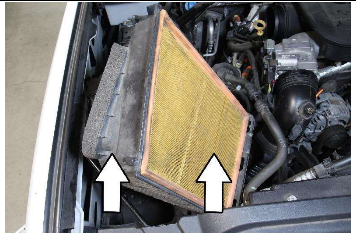
7. Lift up gently and disconnect the lower air box assembly from the rubber grommets. Remove the lower air box assembly from the vehicle.
